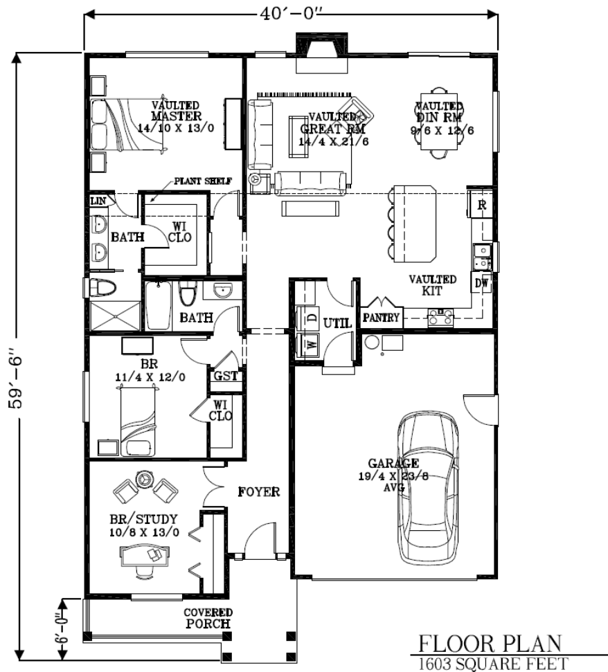
Nehalem M 1603 Square Feet
