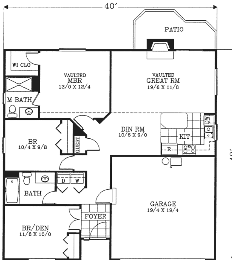
FLOOR PLAN 1192 SQUARE FEET
