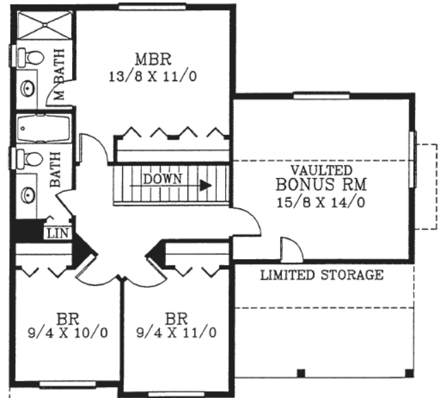
UPPER FLOOR PLAN 654 SQUARE FEET NIC 242 SQ FT BONUS ROOM
